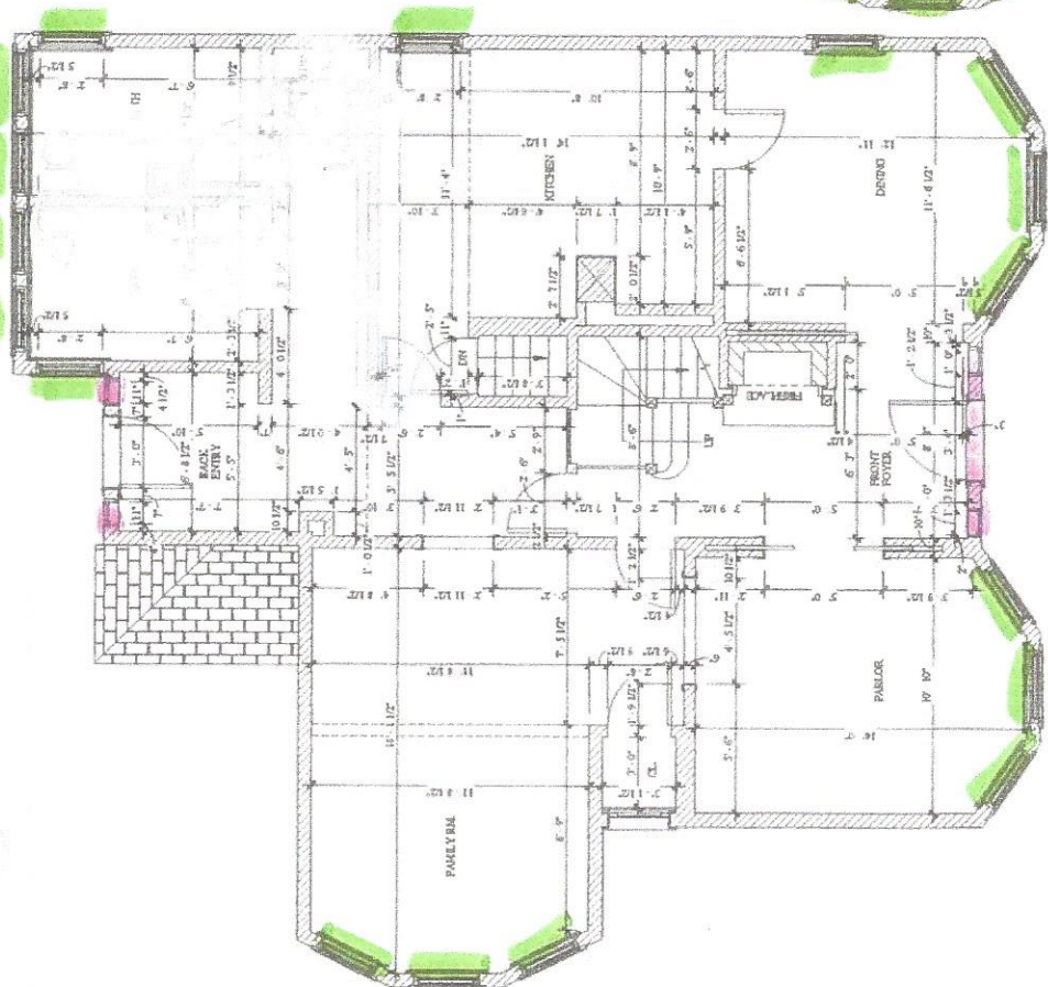
EXISTING 1st FLOOR PLAN 1/4" = 1'-0"
